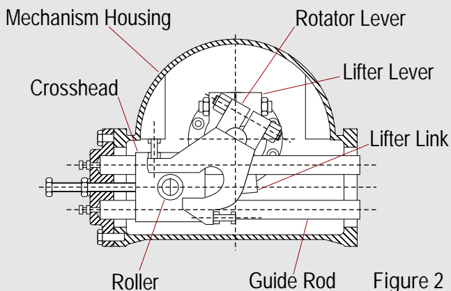
Actuator Mechanism Cross Section
