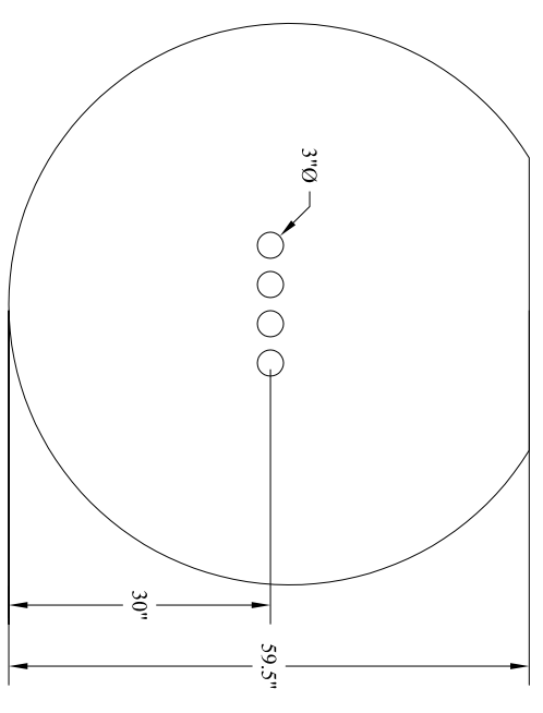
Tank Baffle
